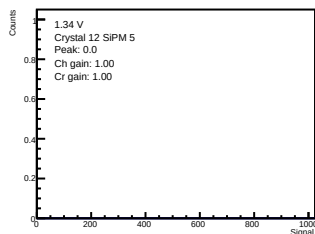
ADC-only | 1.34 V | crystal 12 | sipm 5
