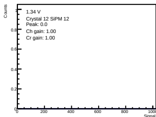
ADC-only | 1.34 V | crystal 12 | sipm 12
